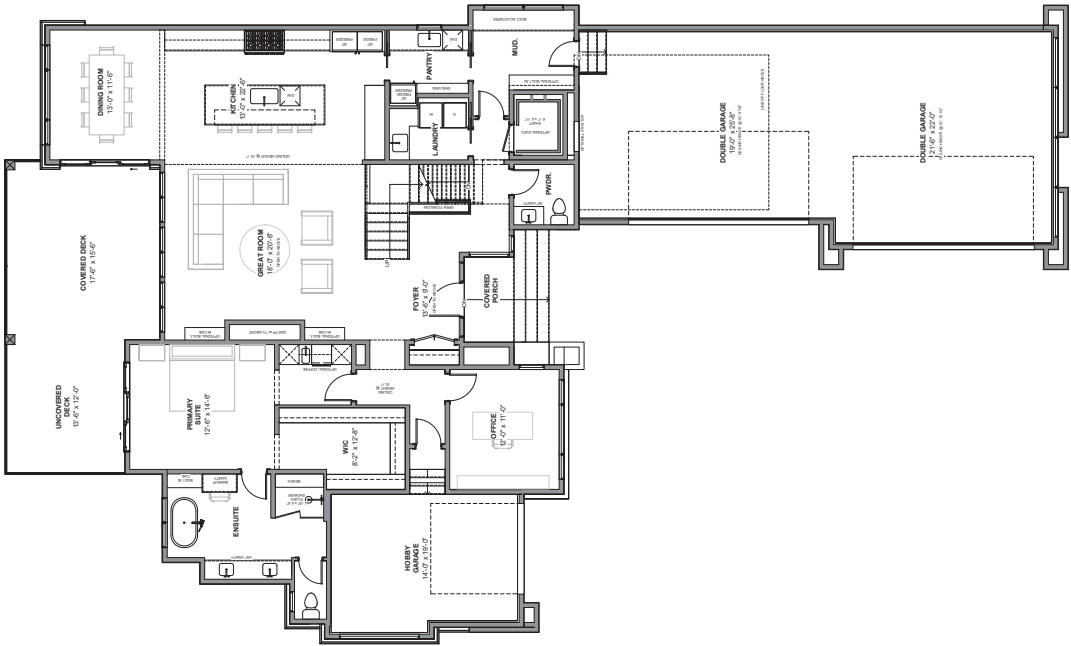
MAIN LEVEL 2183 SQ FT
