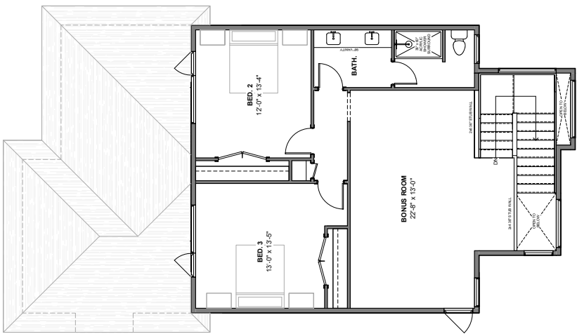
UPPER LEVEL 1078 SQ FT
