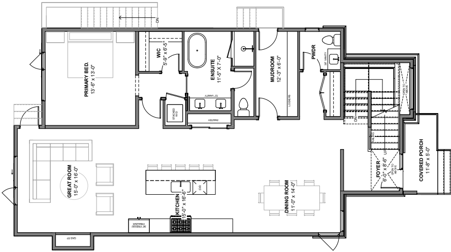
MAIN LEVEL 1559 SQ FT
