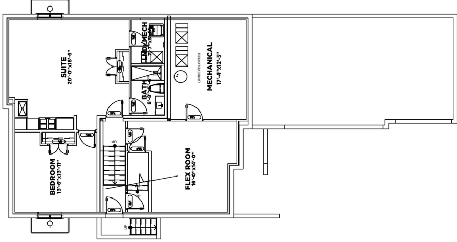
LOWER LEVEL\FLEX ROOM 364 SQ FT SUITE 653 SQ FT
