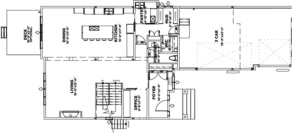
MAIN LEVEL 1401 SQ FT
