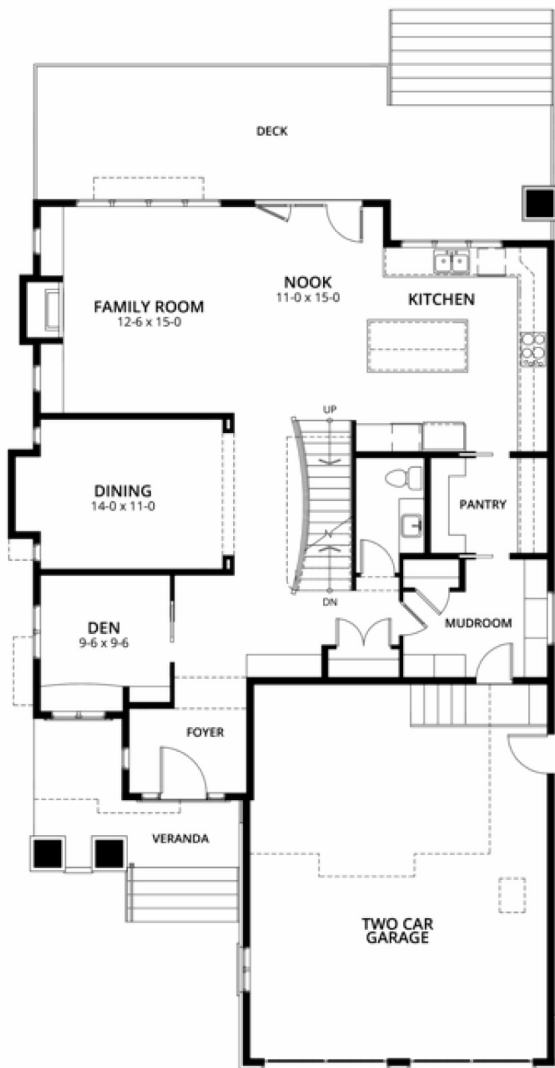
MAIN 1428 Sq. Ft.
